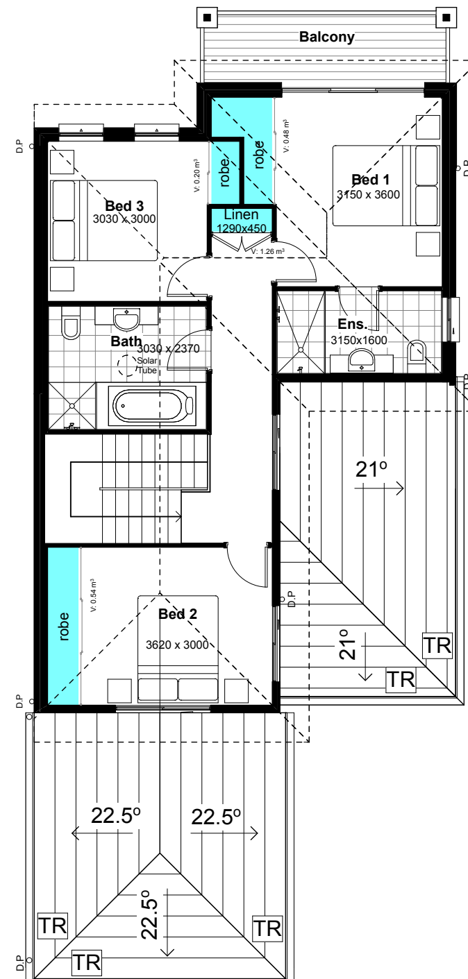
2 First Floor
