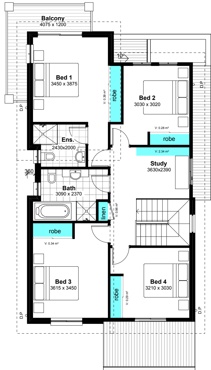
2 First Floor
