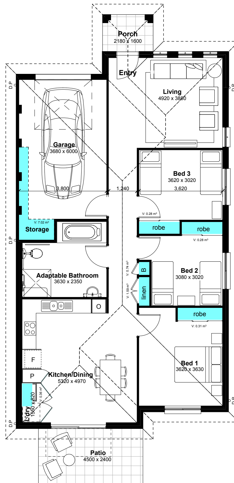
1 Ground Floor
