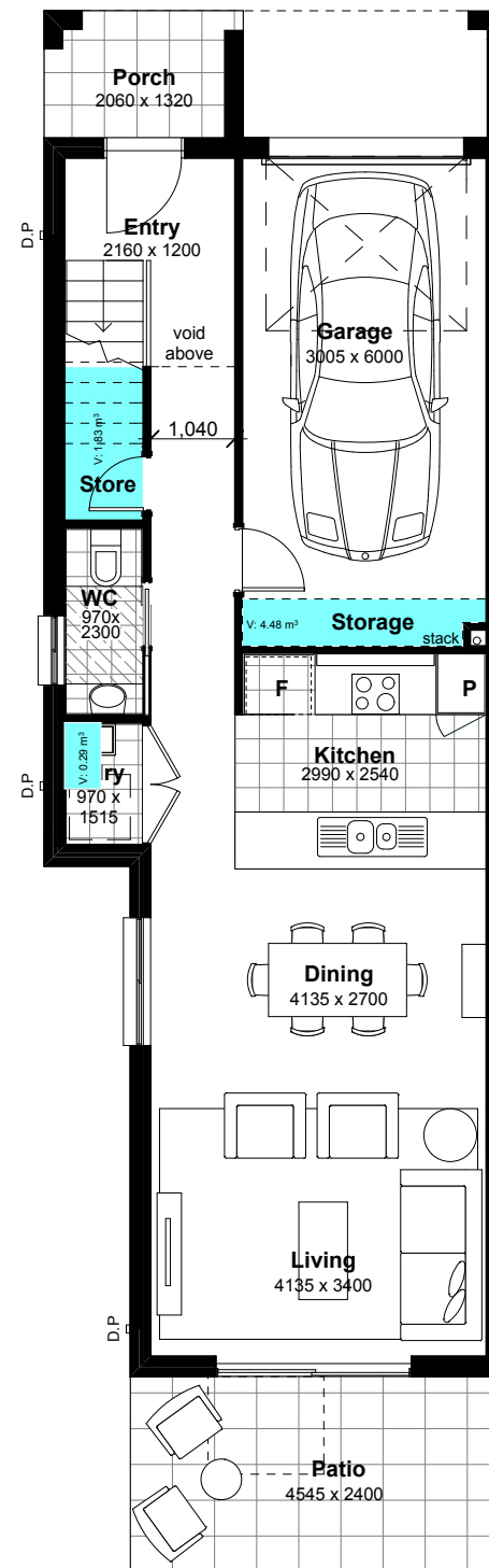
1 Ground Floor
