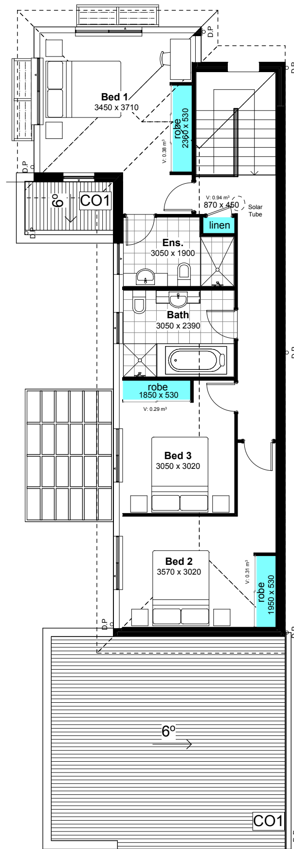
2 First Floor
