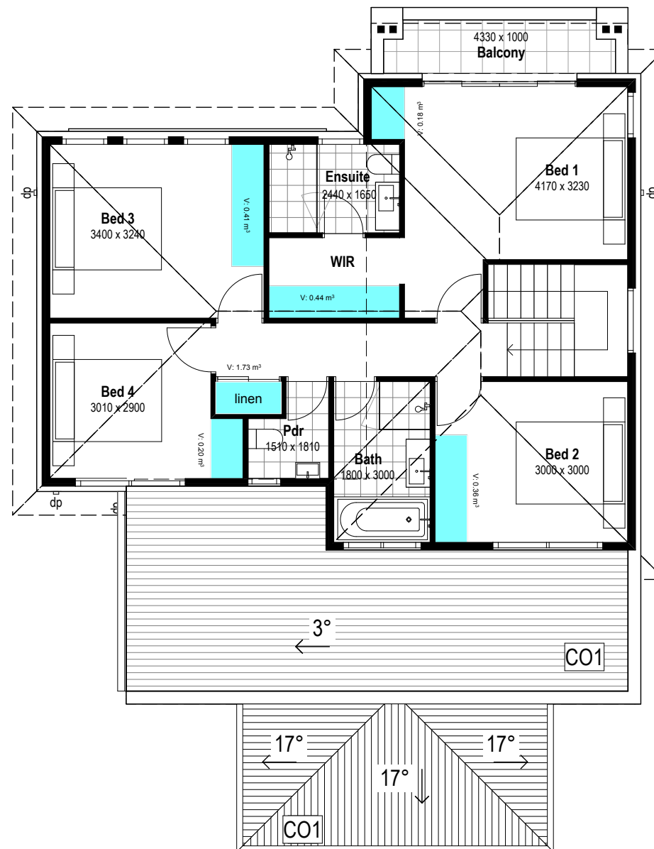
2 First Floor
