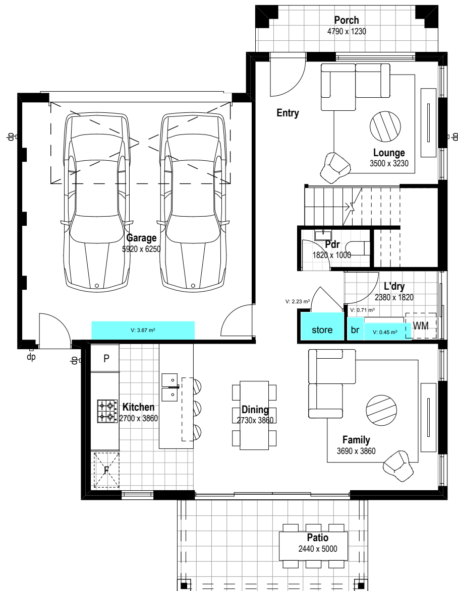
1 Ground Floor
