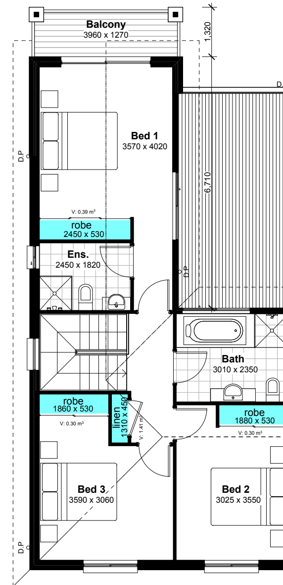
2 First Floor
