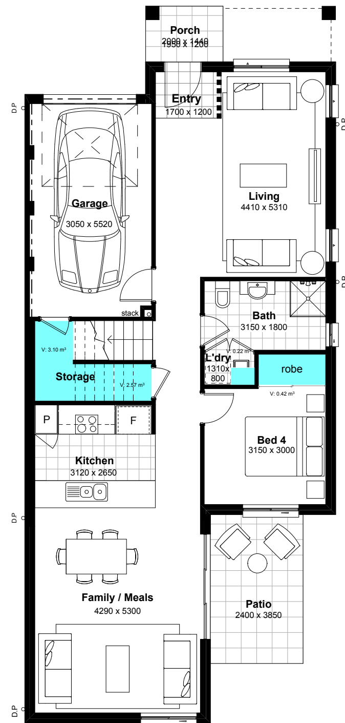
1 Ground Floor
