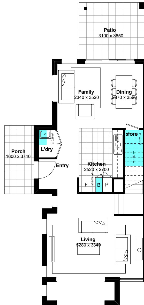
1 Ground Floor
