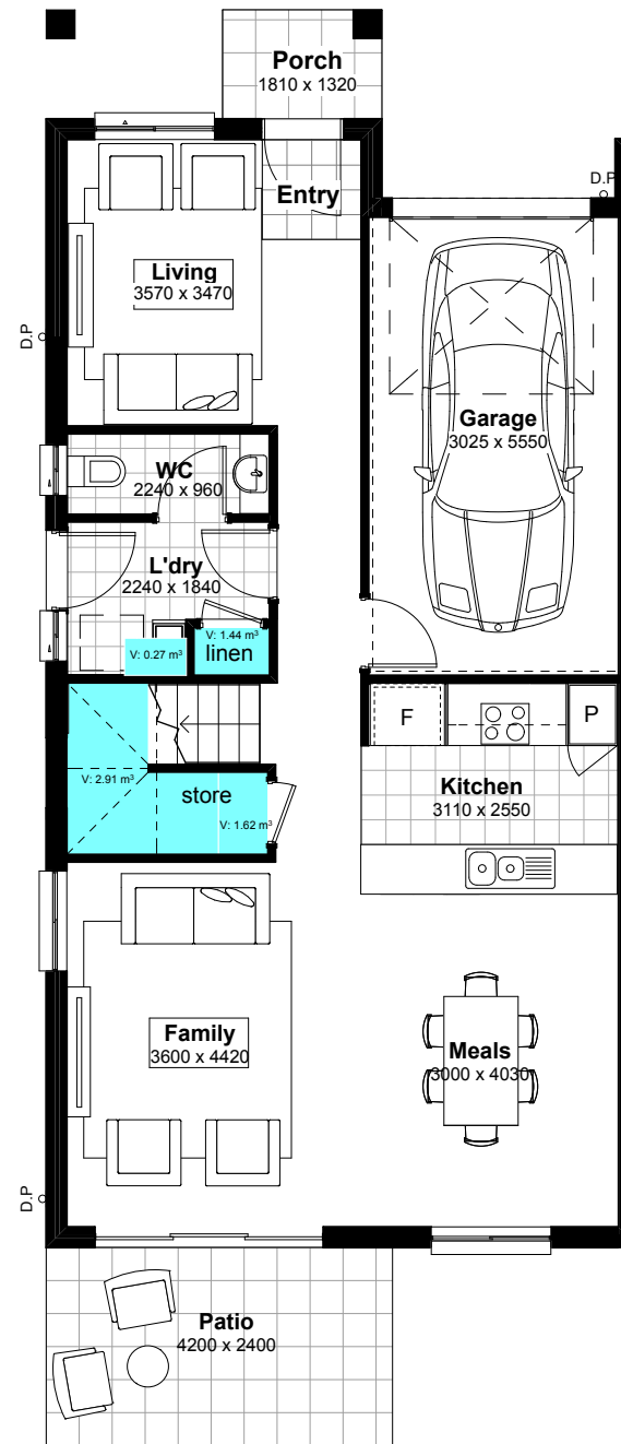
1 Ground Floor
